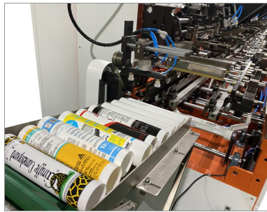
In-feed Conveyor
