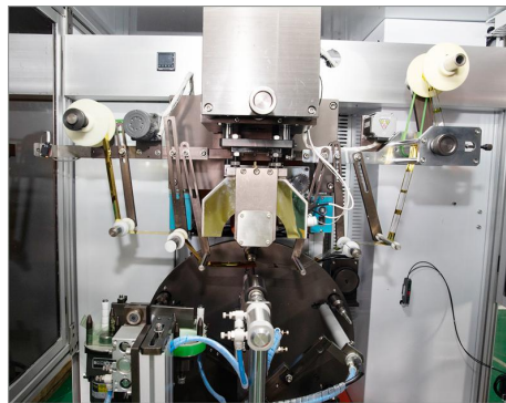
Hot Stamping Station
