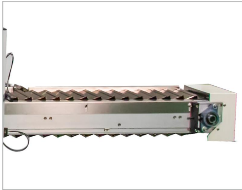
In-feed Conveyor
