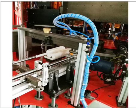
In-feed Conveyor
