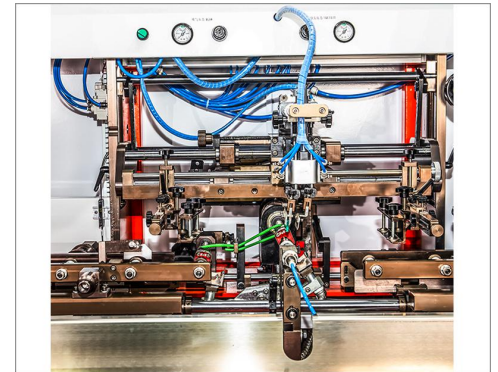
Printing System
